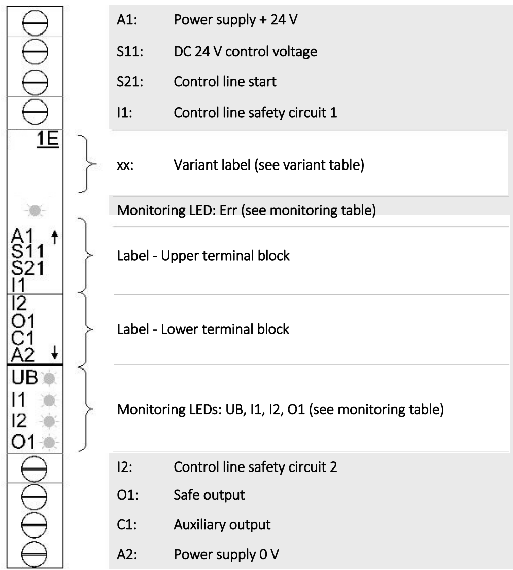
Fig. 8 Front view
