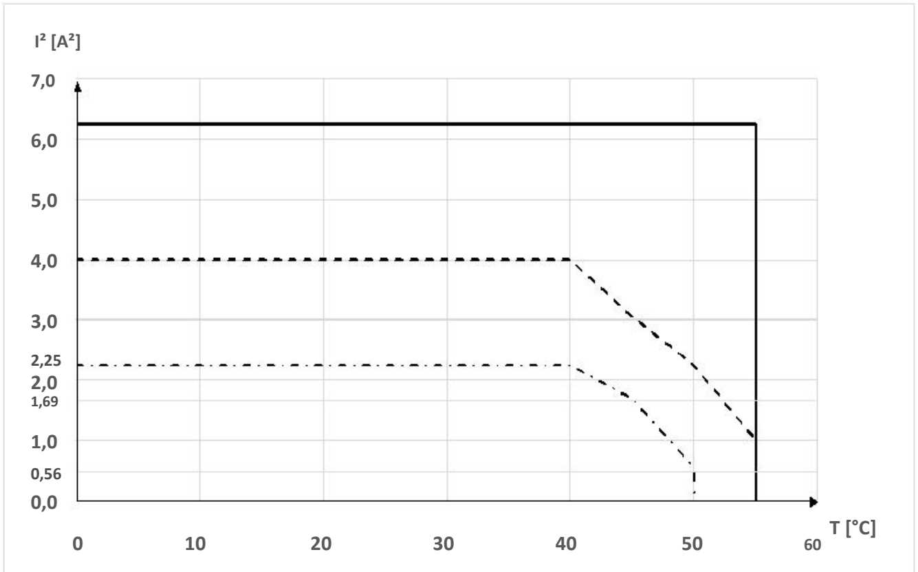
Fig. 26 Derating curve
