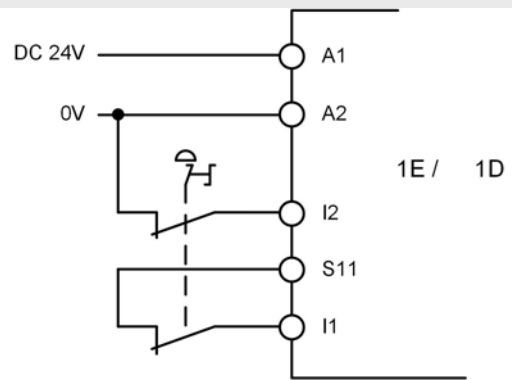
Fig. 9: Potential-free NC contacts dual channel
