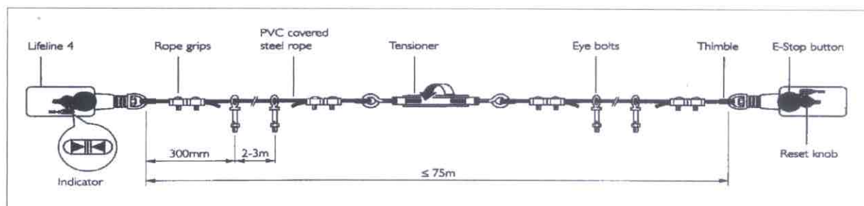
Fig. 3 Mounting specification
