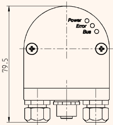
Connection: "T"
