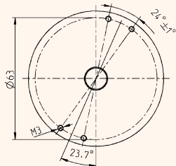
Connection Shaft
