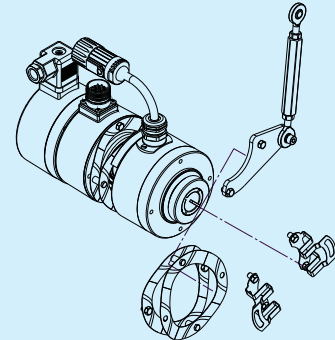
AOSS90 + AINH90xx + FAxH90 with 1 incremental + 1 absolute/ bus output
