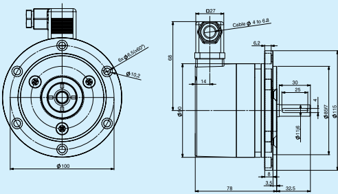
Overspeed switches AOSS9011
