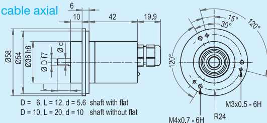
Clamping flange
